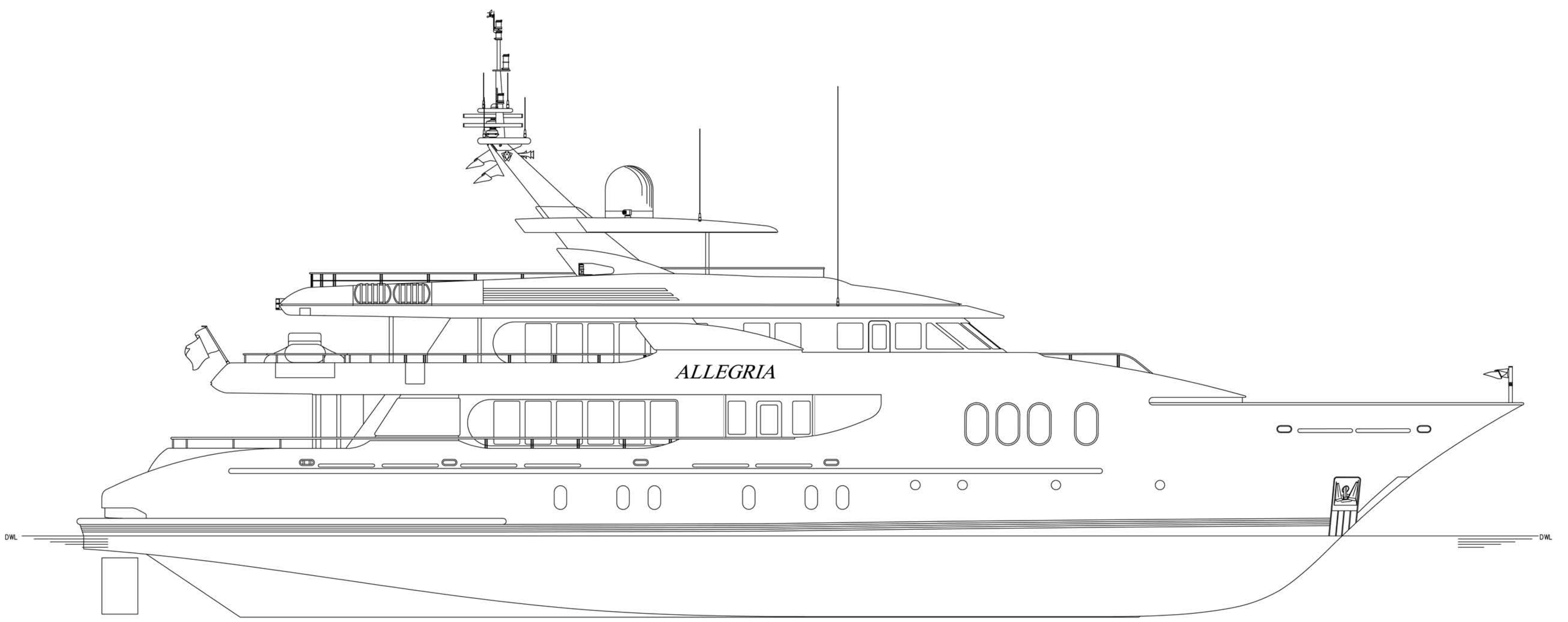
OUTBOARD PROFILE 46 METER
